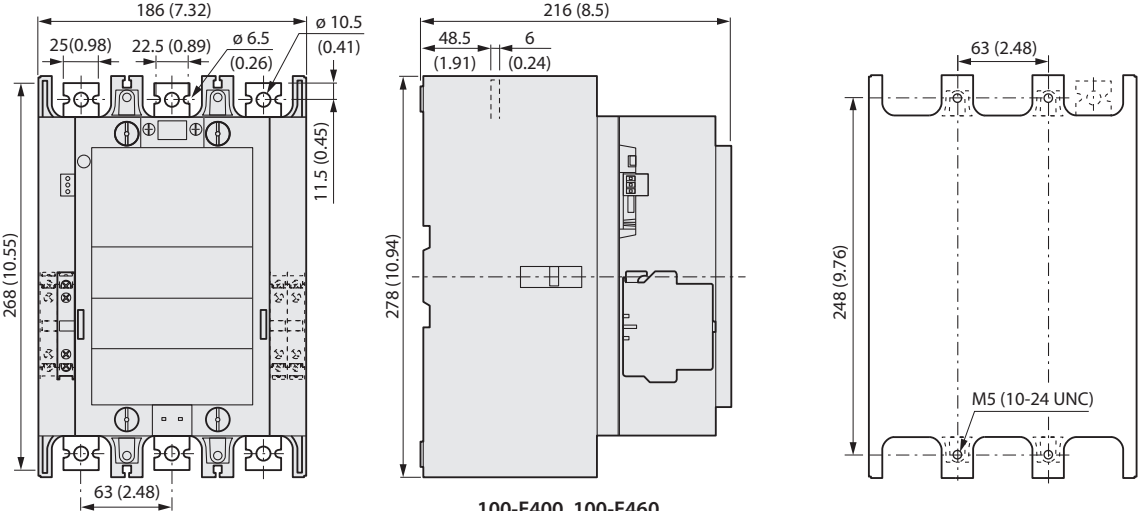
100-E400, 100-E460
